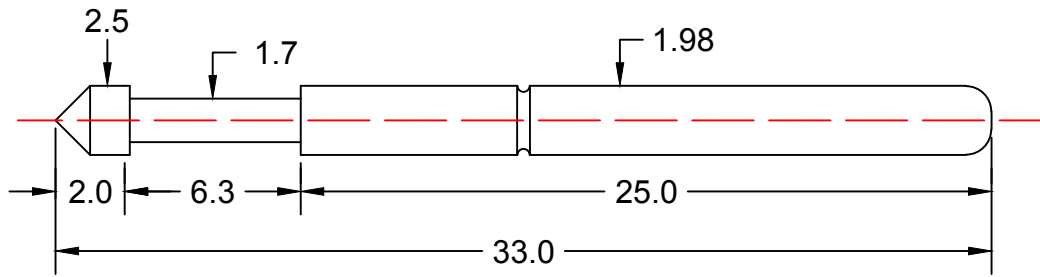
TEX125-E
